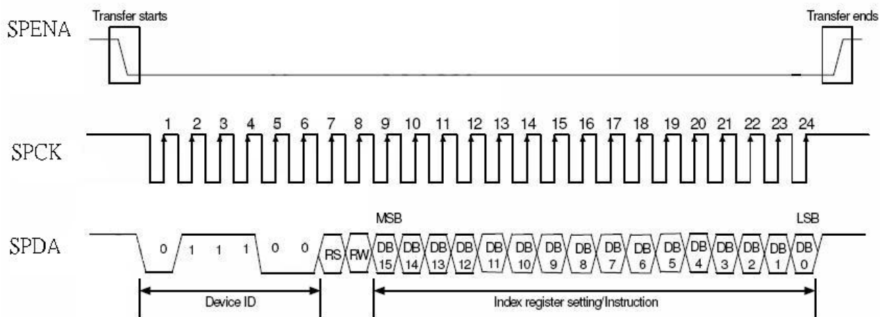
Figure10 SPI timing
