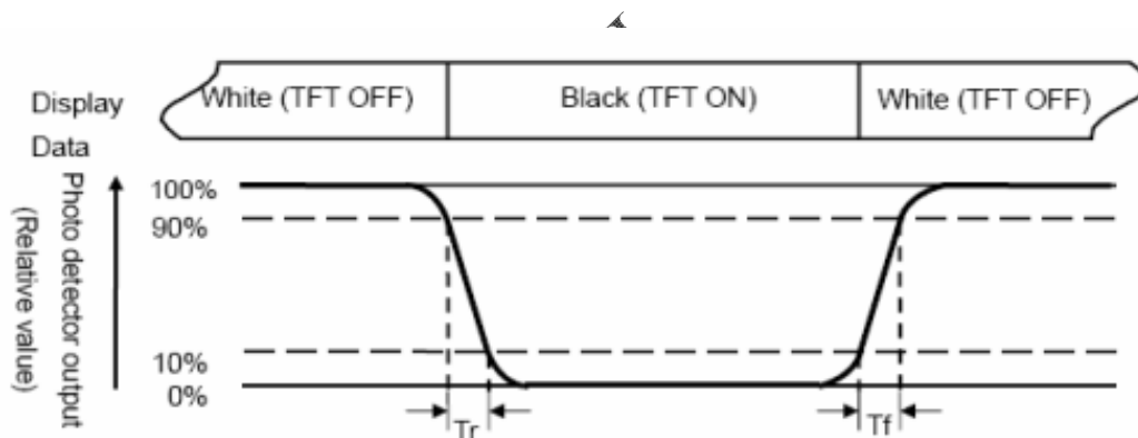
Fig. 3-3 Definition of response time
