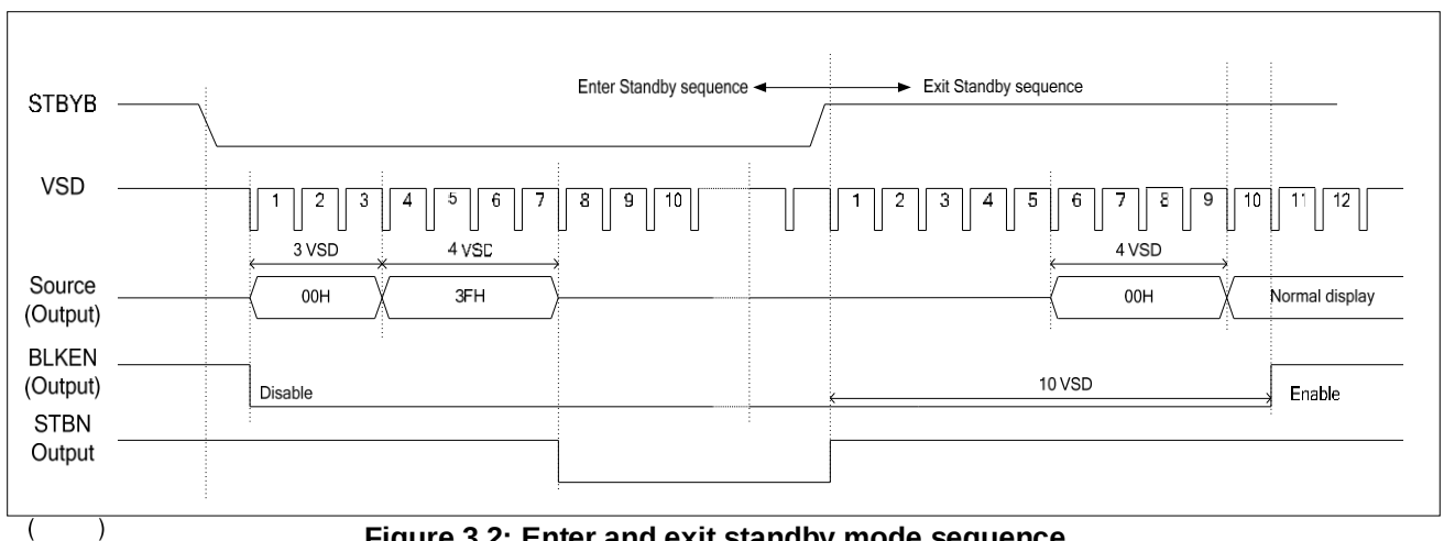
Figure 3.2: Enter and exit standby mode sequence
