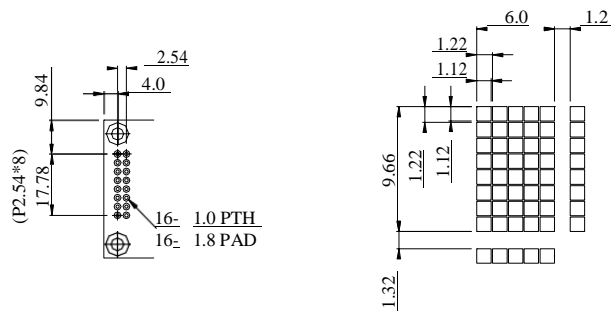
PIN DETAIL
