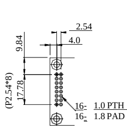
PIN DETAIL
