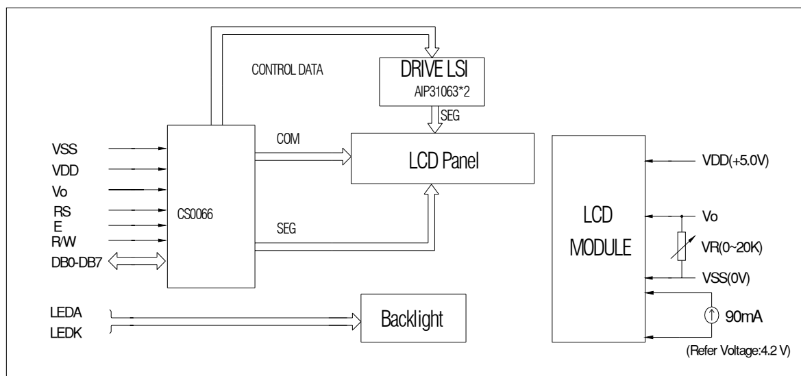
Figure 1. Block diagram
