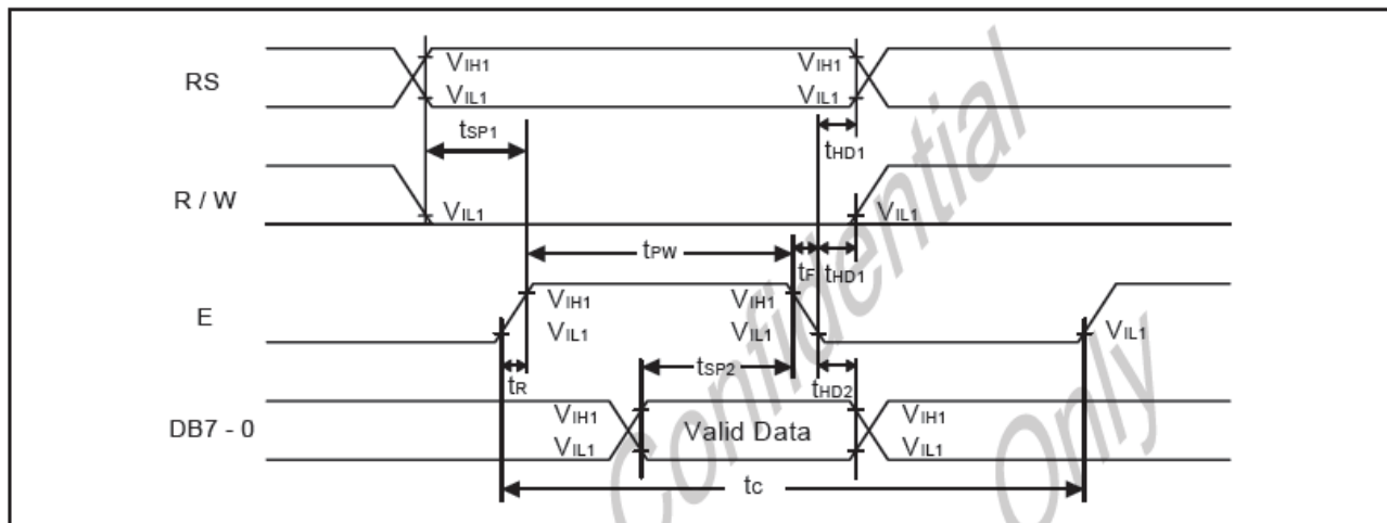
Figure3. Write Mode Timing Diagram
