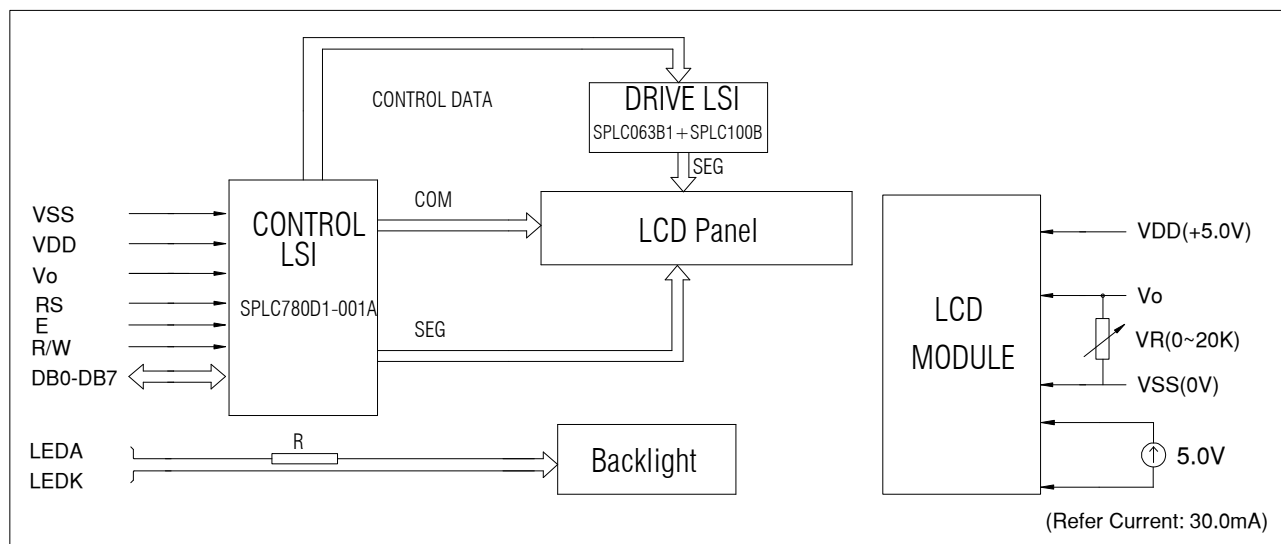
Figure 1. Block diagram
