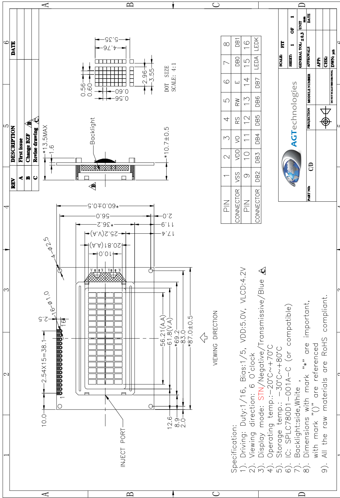
Figure 2. Dimensional outline
