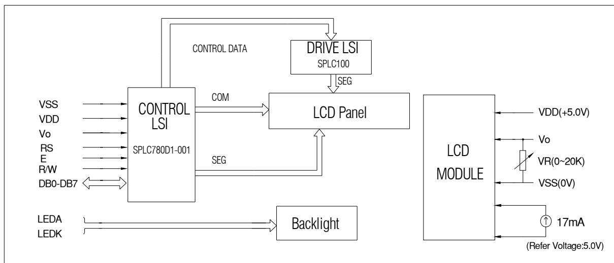
Figure 1. Block diagram
