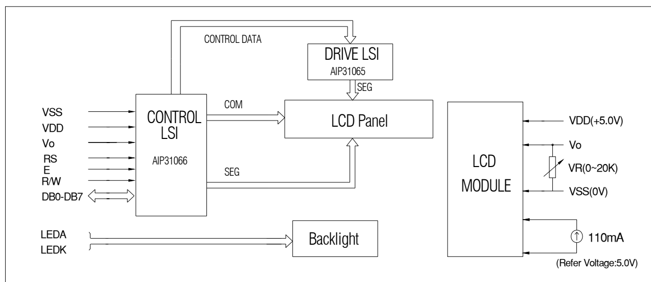
Figure 1. Block Diagram
