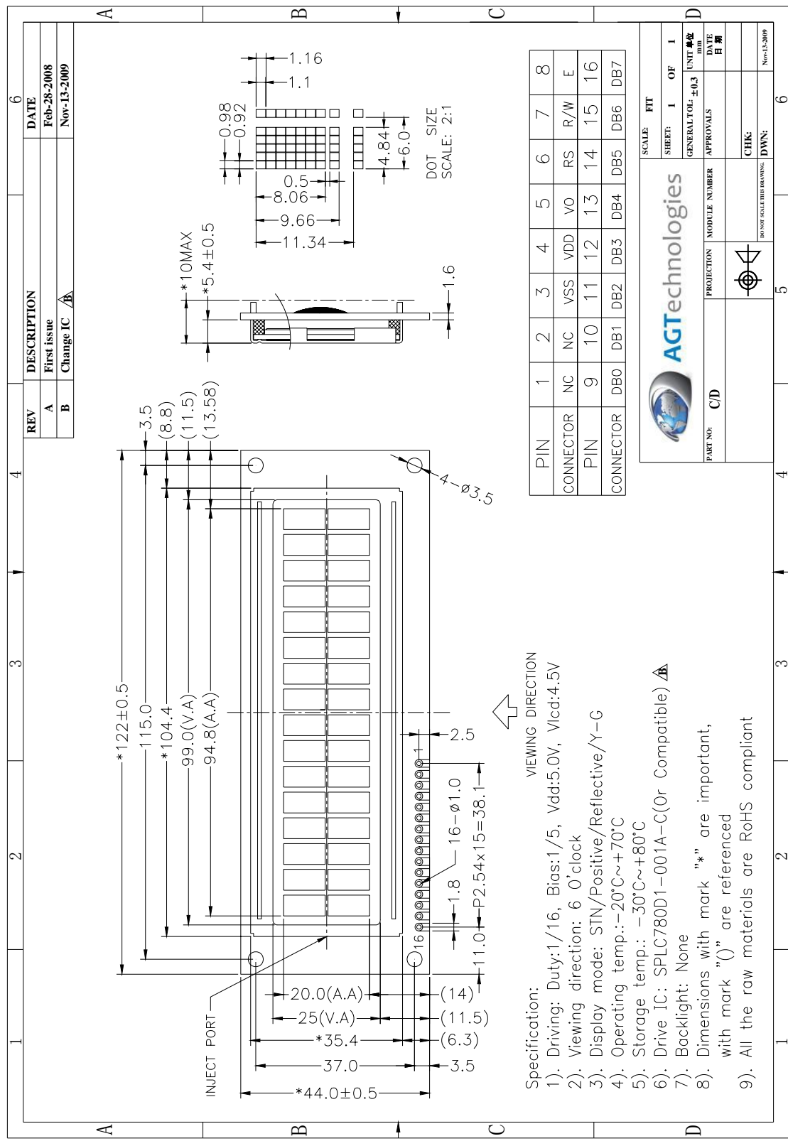
Figure 2. Dimensional outline
